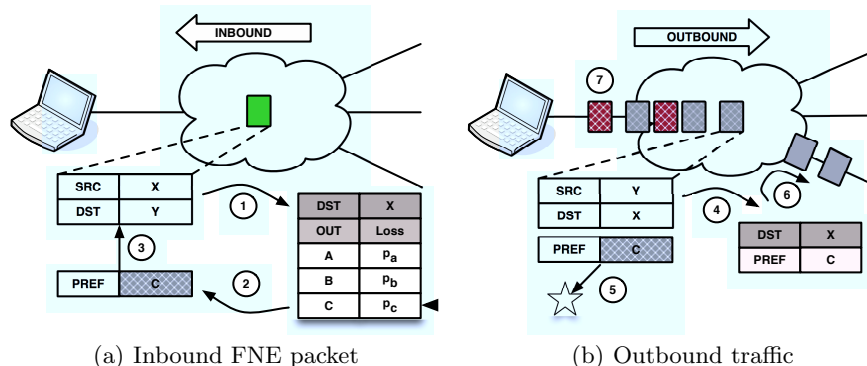
Fig. 1. PREFLEX architecture.
