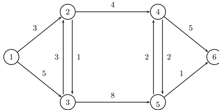
Figure 2: Weighted graph for Dijkstra's algorithm and Bellman-Ford
